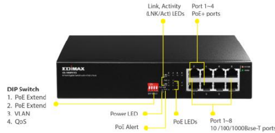
Front Panel
